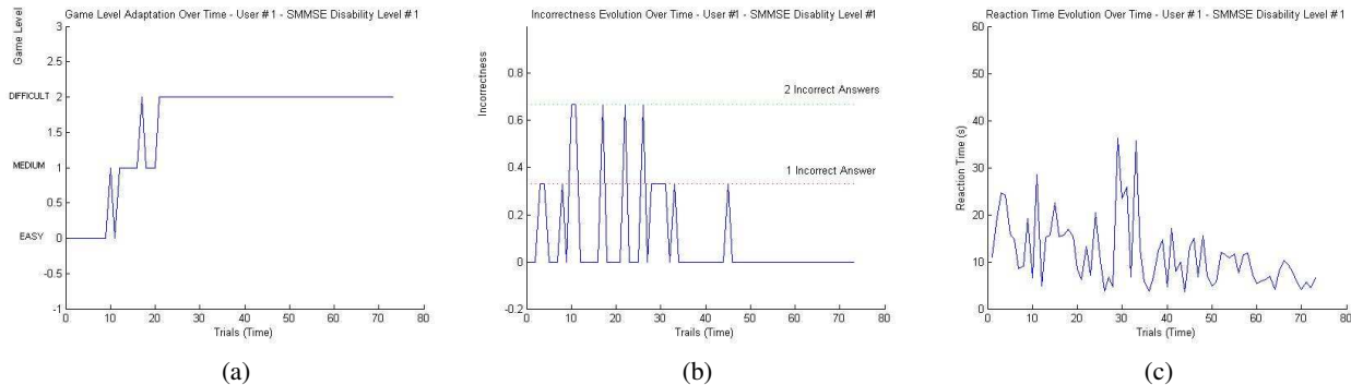
Fig. 4: Results : (a) Game Level Adaptation and Evolution Over Time (6 months) for User Id 1 ; (b) Incorrectness Evolution Over Time (6 months) for User Id 1 ; (c) Reaction Time Evolution Over Time (6 months) for User Id 1
